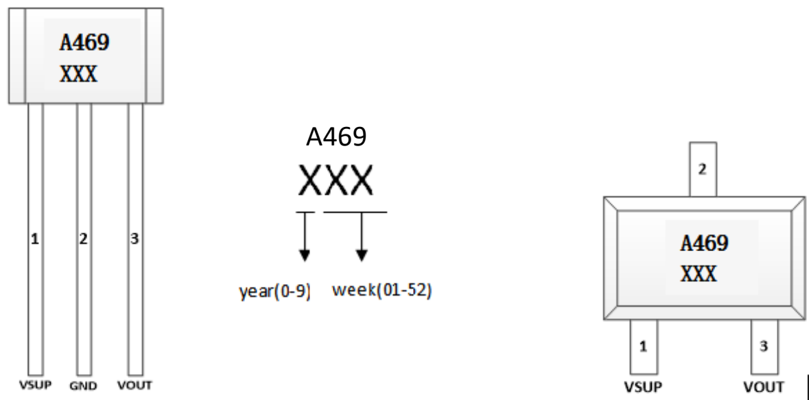
TO92S
