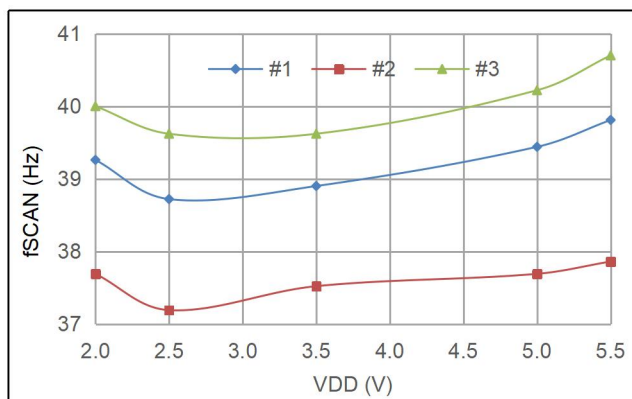
扫描频率 vs. VDD
