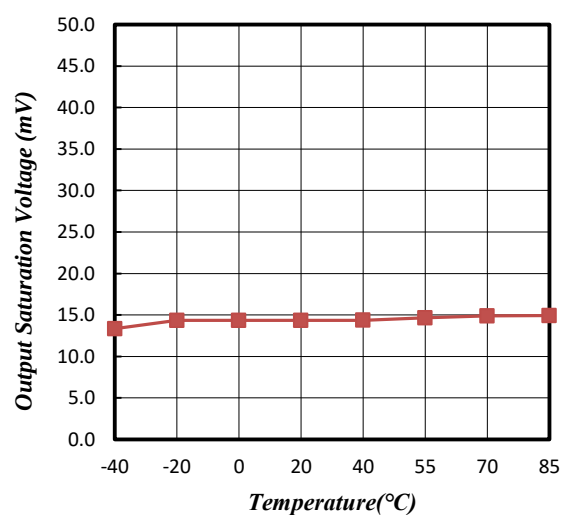
Typical Temperature(TA) Versus Output Voltage(VDS0N)
