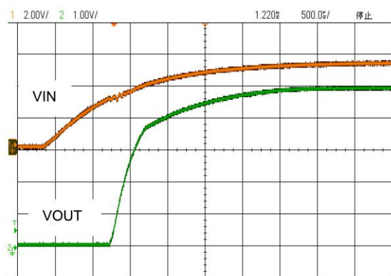
图 15 软启动, V_{IN} = 5.3V , V_{OUT} = 5.0V , I_O = 1.5A
