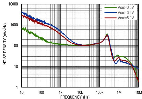
图 11 输出噪声谱密度, V_{IN} = 5V , V_{OUT} = 3.3V
