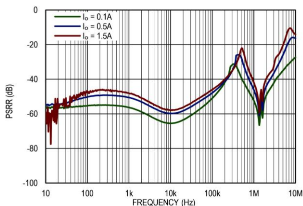
图 14 PSRR, V_{IN} = 5.3V , V_{OUT} = 5.0V
