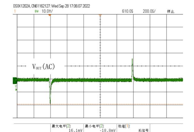
图 24 负载瞬态响应, V_{IN} = 4.3V , V_{OUT} = 3.3V , I_{OUT} = 1mA \sim 1A
