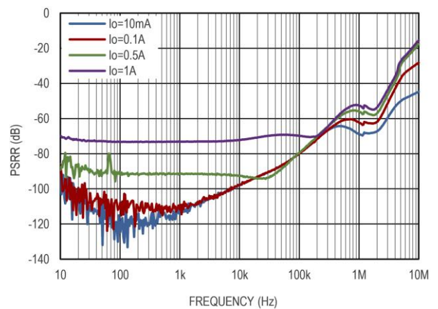
图 22 电源电压纹波抑制比, V_{IN} = 5V , V_{OUT} = 3.3V
