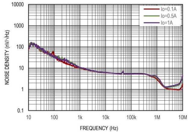
图 20 输出噪声谱密度, V_{IN} = 5V , V_{OUT} = 3.3V
