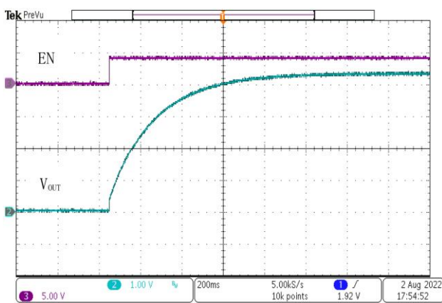
图 23 软启动, V_{IN} = 4.3V , V_{OUT} = 3.3V , I_{OUT} = 1A
