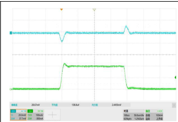
图 26 负载瞬态响应, V_{IN} = 4.3V , V_{OUT} = 3.3V , I_{OUT} = 1mA \sim 200mA
