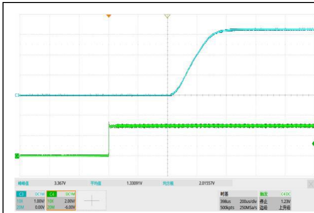
图 25 软启动, V_{IN} = 4.3V , V_{OUT} = 3.3V , I_{OUT} = 300mA
