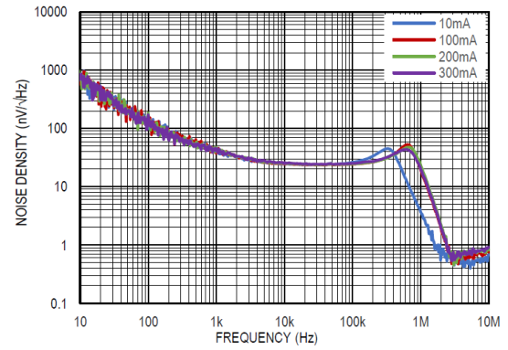
图 18 输出噪声谱密度, V_{IN} = 5V , V_{OUT} = 3.3V
