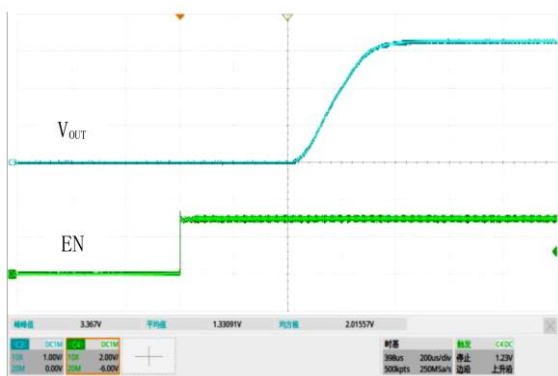
图 23 软启动, V_{IN} = 4.3V , V_{OUT} = 3.3V , I_{OUT} = 300mA
