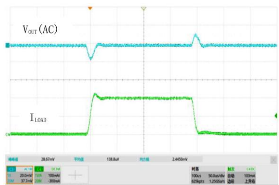
图 24 负载瞬态响应, V_{IN} = 4.3V , V_{OUT} = 3.3V , I_{OUT} = 1mA \sim 200mA
