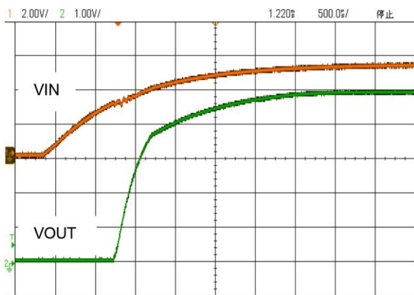
图23 软启动, V_{IN} = 5.3V , V_{OUT} = 5.0V , I_O = 3A
