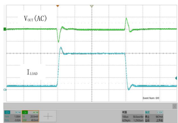
图24 负载跳变, V_{IN} = 2.8V , V_{OUT} = 1.8V , I_O = 0.3A \sim 3A
