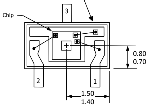
Bottom View of SOT-23
