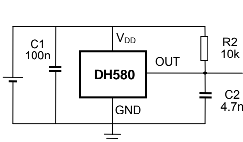
Typical Three-Wire Application Circuit
